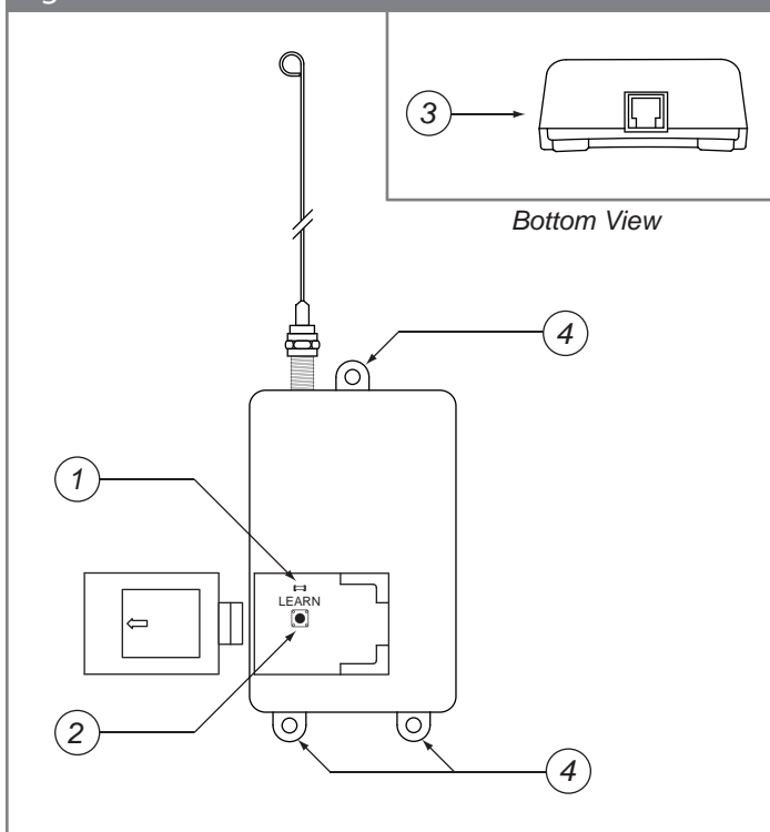
Figure 2: Receiver
