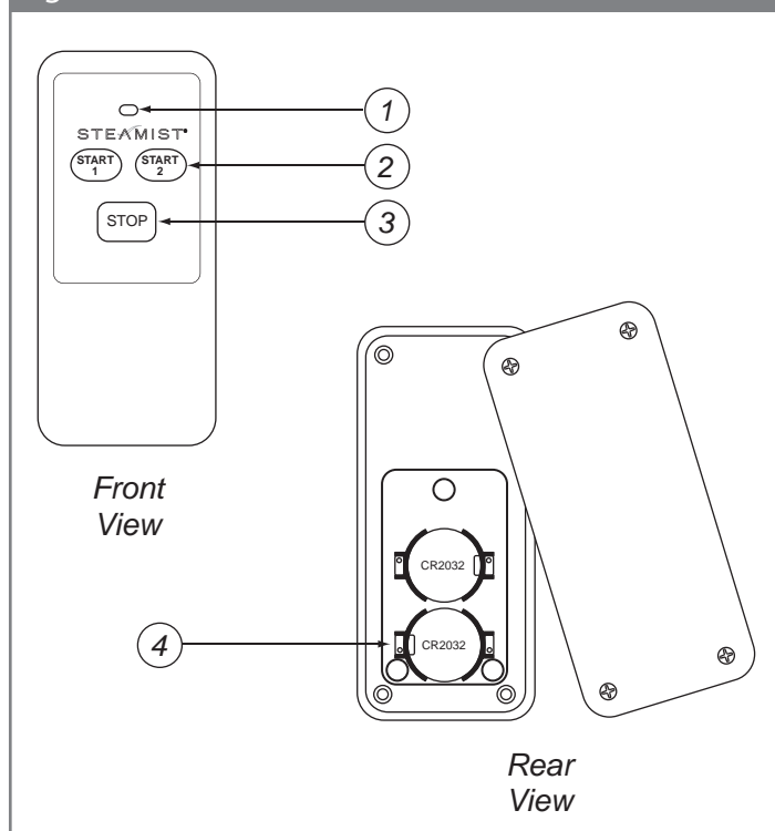
Figure 1: Remote Control
